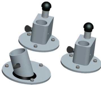
SPA2001-18 - Spiked manhole guard feet
